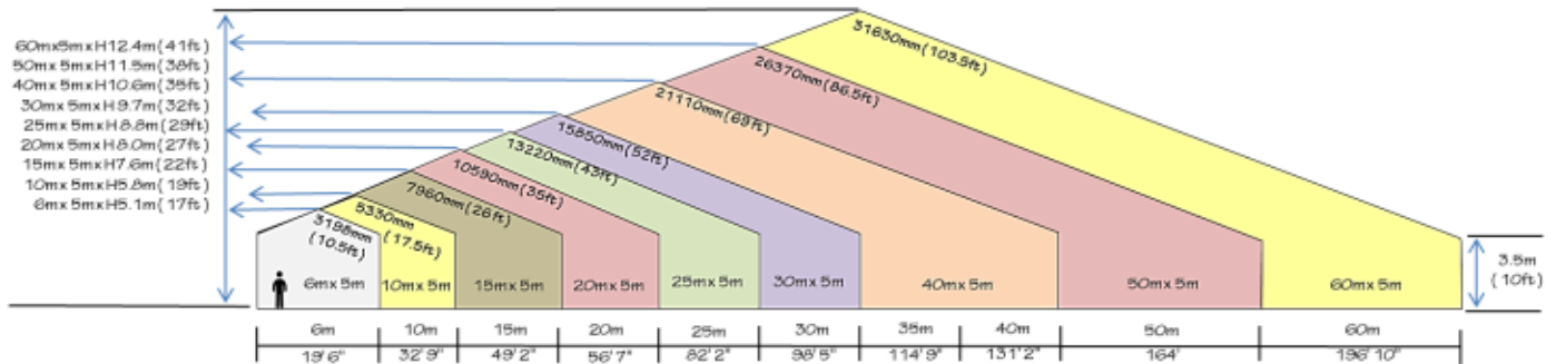
Marquee Tent 10m x 5m (2 block)
