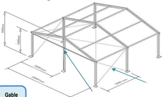
Gable Frame 15m
